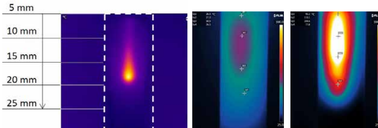
During drilling of the bone samples, temperature elevation can be continuously monitored at any drilling depth and different drill bit designs and process parameters were investigated and subsequently optimized.
