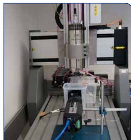
A 3Dof test rig for bone drilling integrated with FLIR thermal imaging was set up in order to measure the temperature increase in the skull as a result of the drilling process.
